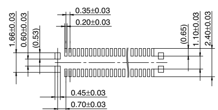
Recommended metal mask pattern Metal mask thickness: When 120µm (Terminal opening ratio: 70%) (Metal-part opening ratio: 100%)
