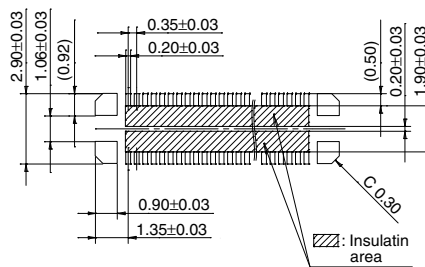
Recommended metal mask pattern Metal mask thickness: When 120µm (Terminal opening ratio: 70%) (Metal-part opening ratio: 100%)
